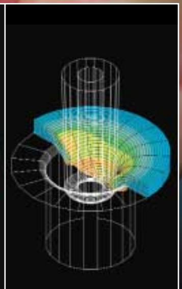
Stresses in membrane during luer insertion
