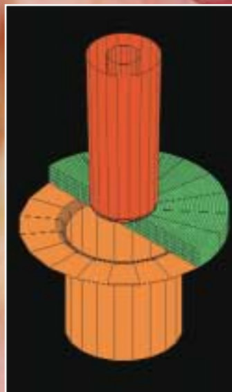
Hyperelastic finite element model of luer insertion into elastomer membrane.
