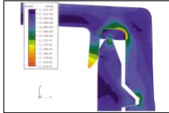
Stress relaxation, seal contact pressure and leakage analysis in a plastic closure during autoclave sterilization.
